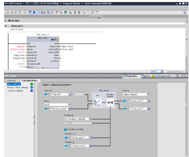
PID 3-Step in the program editor with S7-1200
