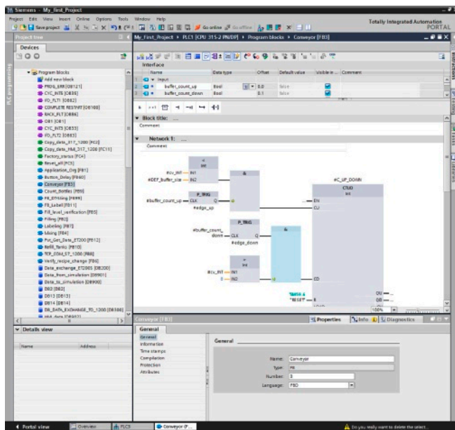
Function Block Diagram (FBD) editor
