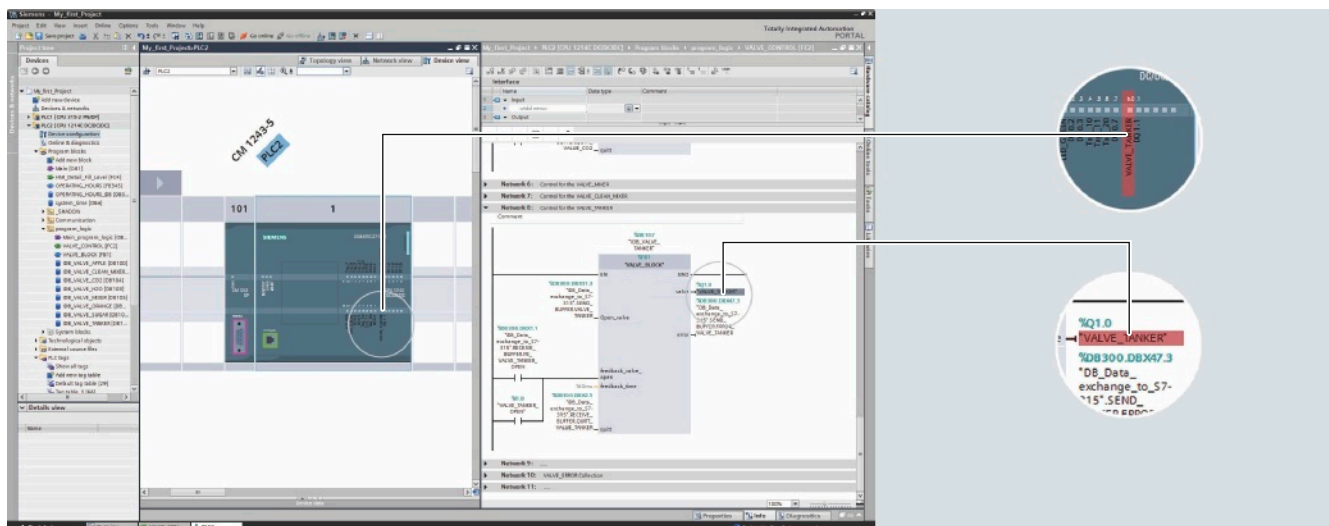
Symbolic programming
