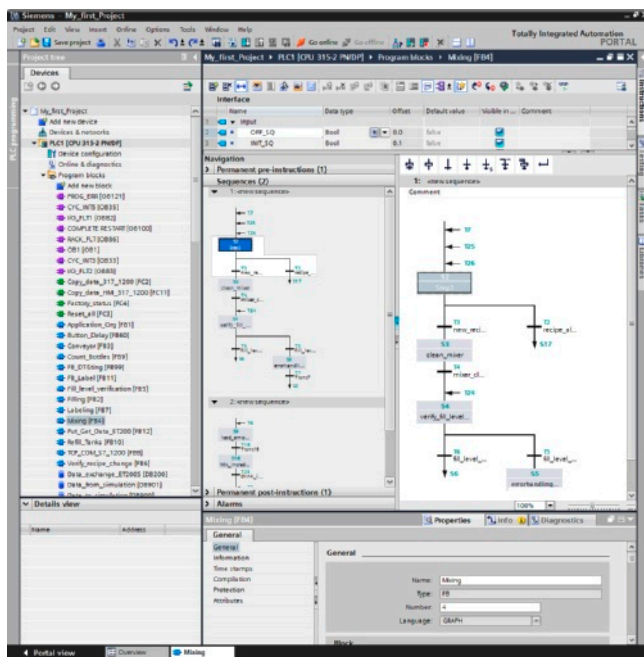
S7-GRAPH Editor
